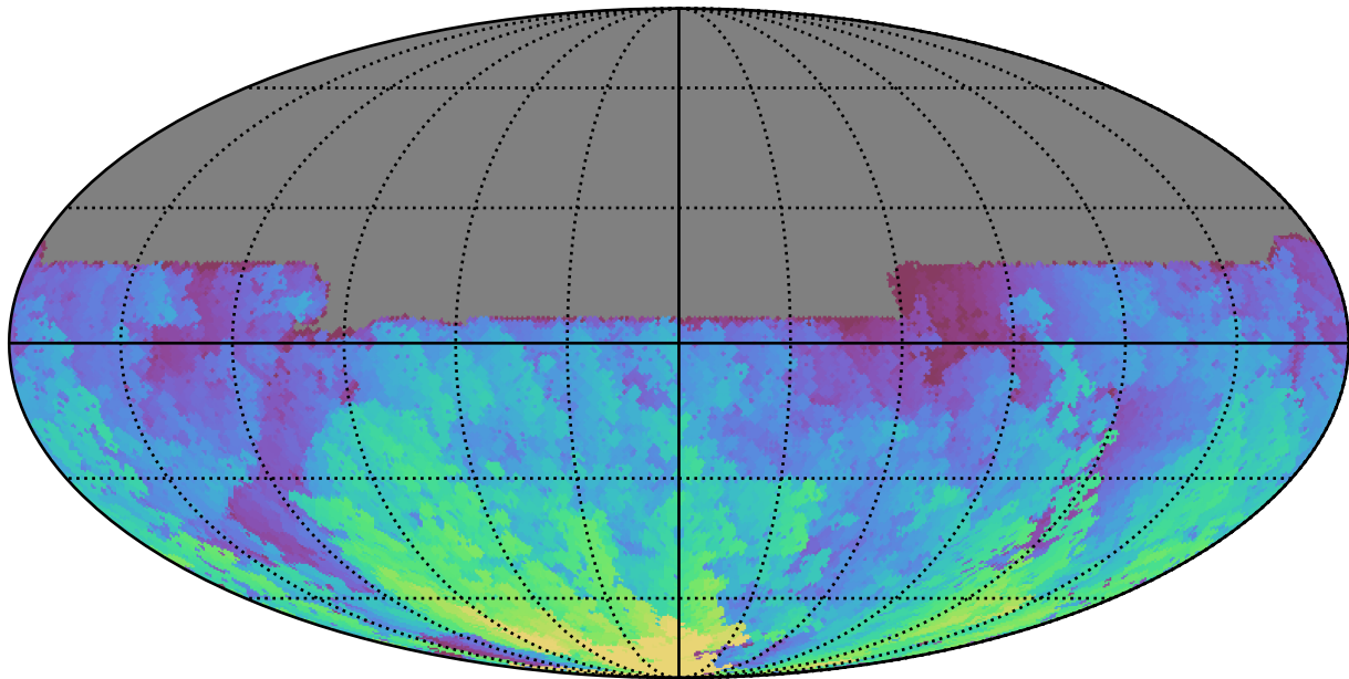
too_elab_2yr_r128_d3_griz_v3.4_10yrs All sky u band: Max HA
