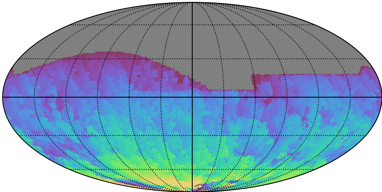
too_elab_2yr_r128_d3_griz_v3.4_10yrs All sky r band: Max HA
