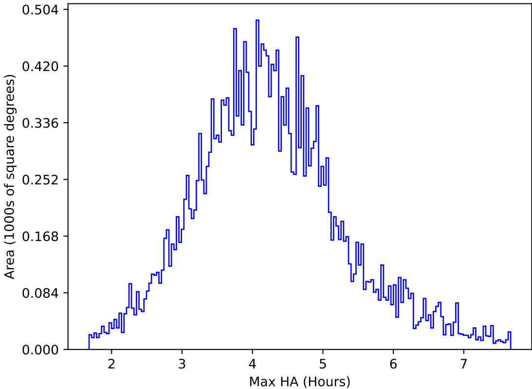
too_elab_2yr_r128_d3_griz_v3.4_10yrs All sky r band: Max HA
