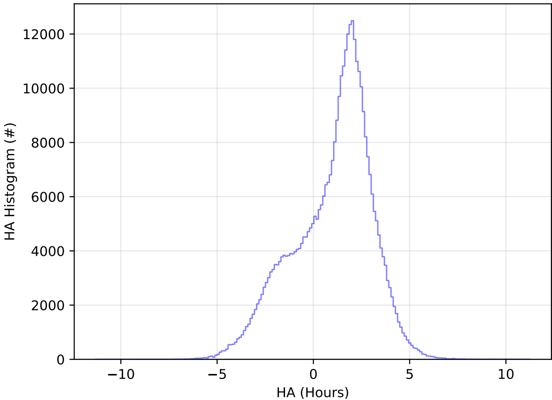
too_elab_2yr_r128_d3_griz_v3.4_10yrs WFD y band: HA Histogram
