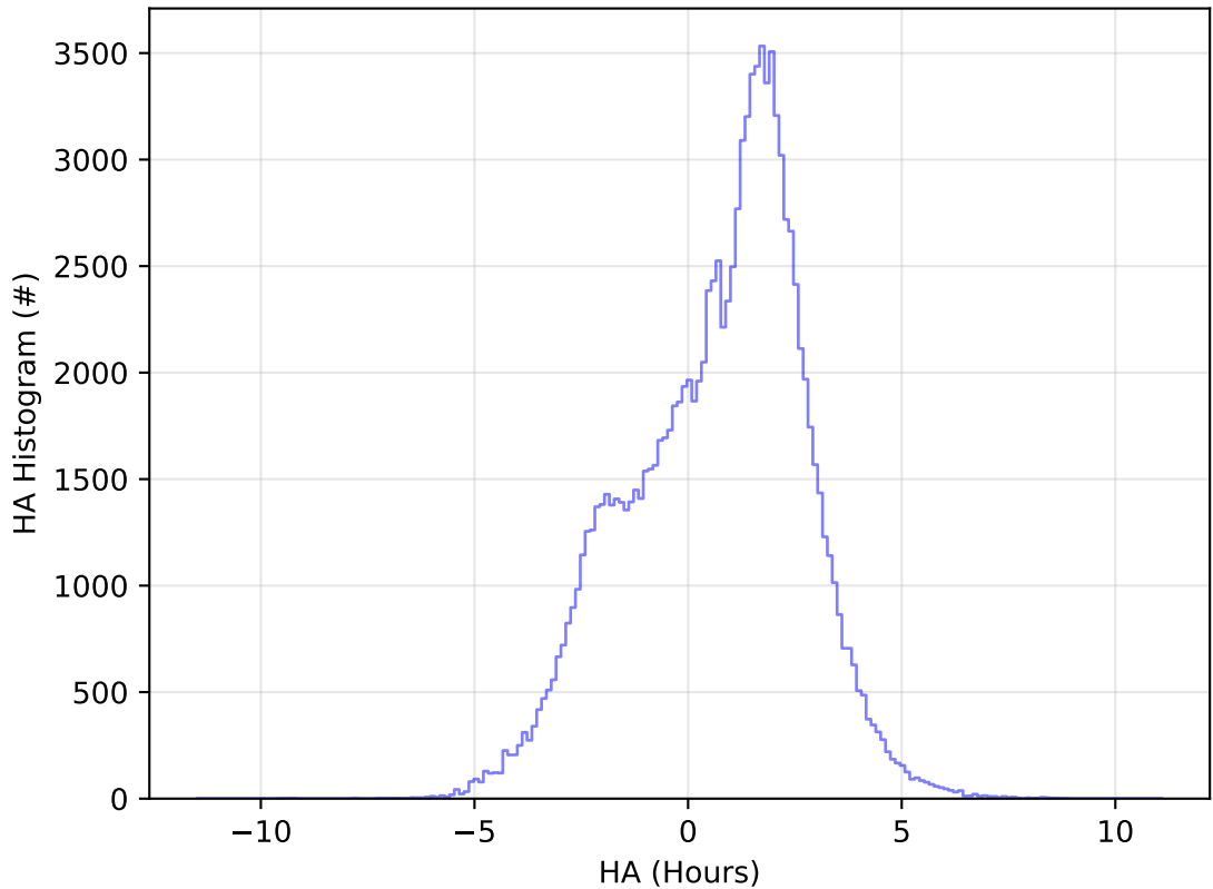
too_elab_2yr_r128_d3_griz_v3.4_10yrs WFD u band: HA Histogram
