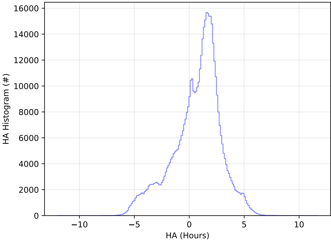
too_elab_2yr_r128_d3_griz_v3.4_10yrs WFD i band: HA Histogram
