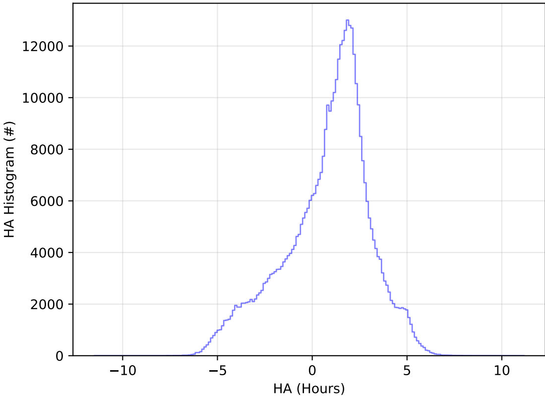
too_elab_2yr_r128_d3_griz_v3.4_10yrs All sky z band: HA Histogram
