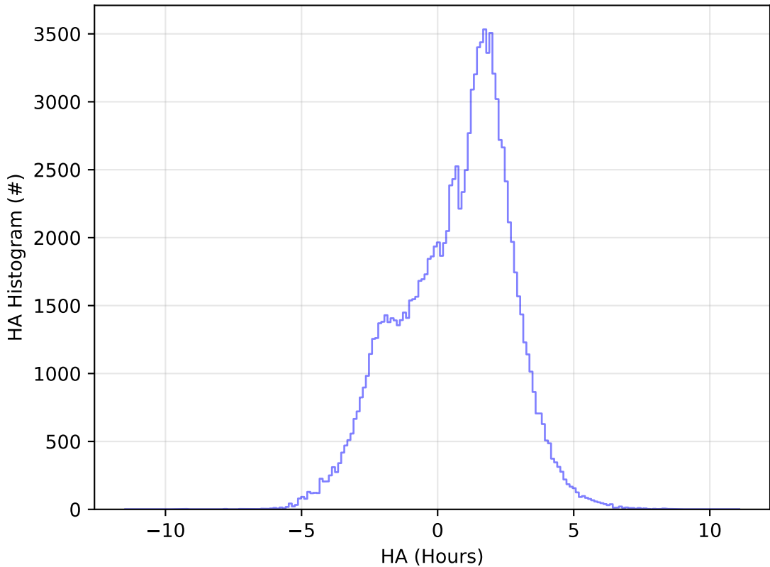
too_elab_2yr_r128_d3_griz_v3.4_10yrs All sky u band: HA Histogram
