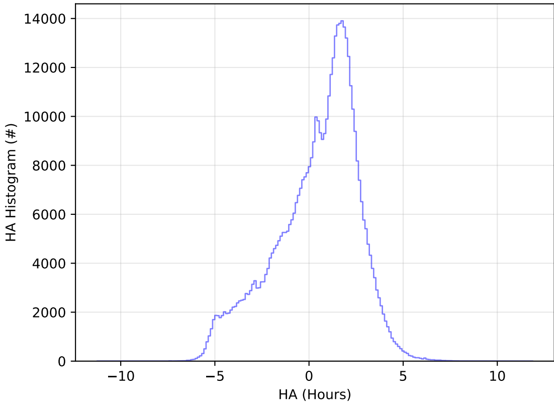
too_elab_2yr_r128_d3_griz_v3.4_10yrs All sky r band: HA Histogram
