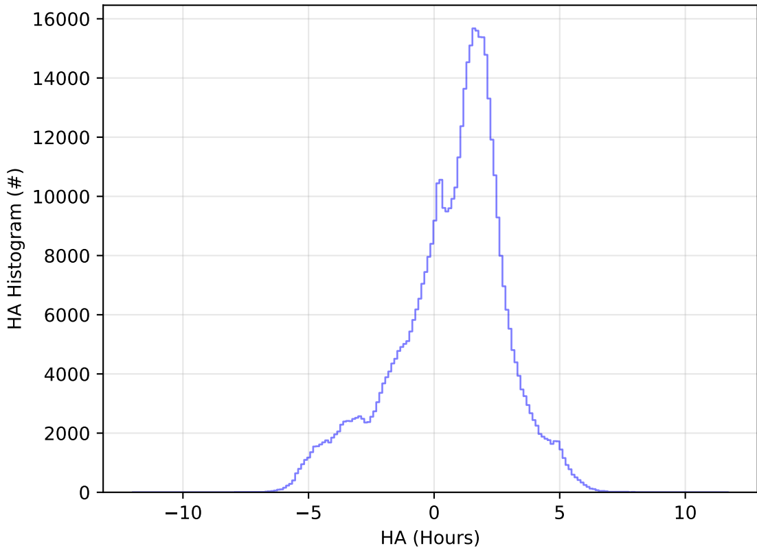
too_elab_2yr_r128_d3_griz_v3.4_10yrs All sky i band: HA Histogram
