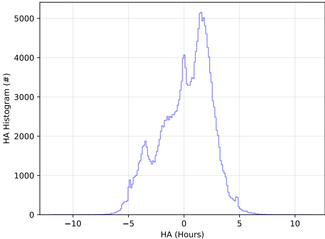
too_elab_2yr_r128_d3_griz_v3.4_10yrs All sky g band: HA Histogram
