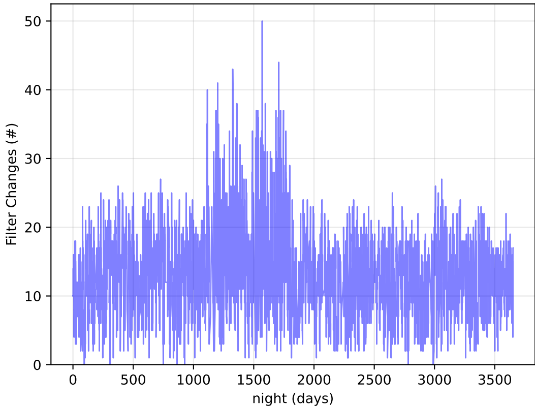
too_elab_2yr_r128_d3_griz_v3.4_10yrs Per Night: Filter Changes
