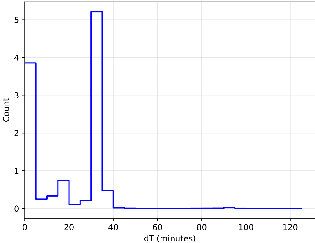
too_elab_2yr_r128_d3_griz_v3.4_10yrs WFD: DeltaT Histogram 1e6
