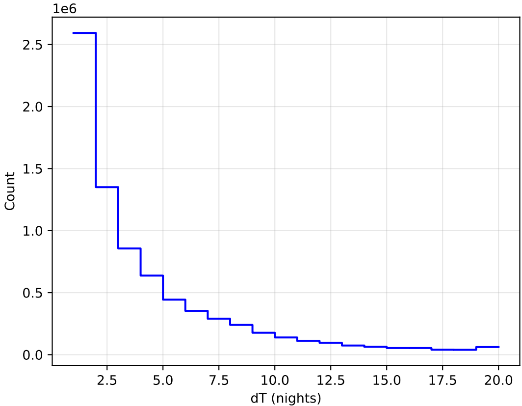
too_elab_2yr_r128_d3_griz_v3.4_10yrs WFD all bands: DeltaNight Histogram
