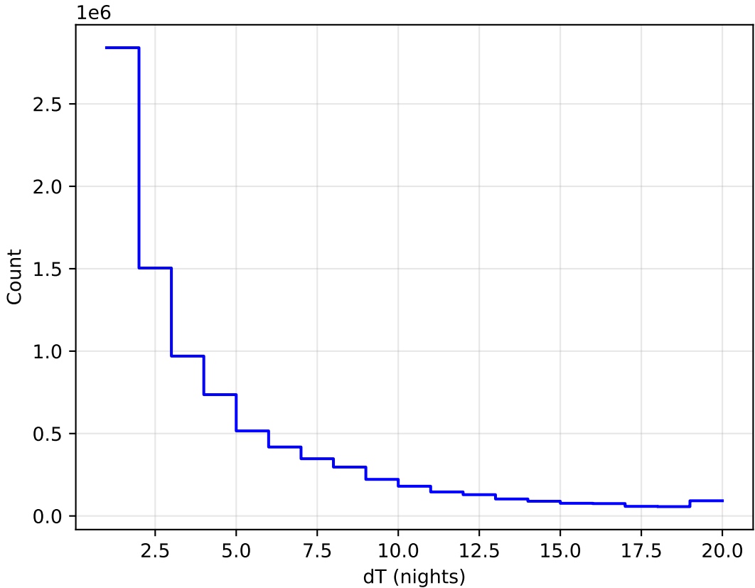
too_elab_2yr_r128_d3_griz_v3.4_10yrs All sky all bands: DeltaNight Histogram
