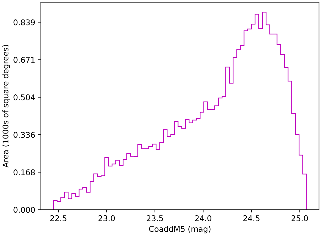
too_elab_2yr_r128_d3_griz_v3.4_10yrs Yr 3-4 z band: CoaddM5
