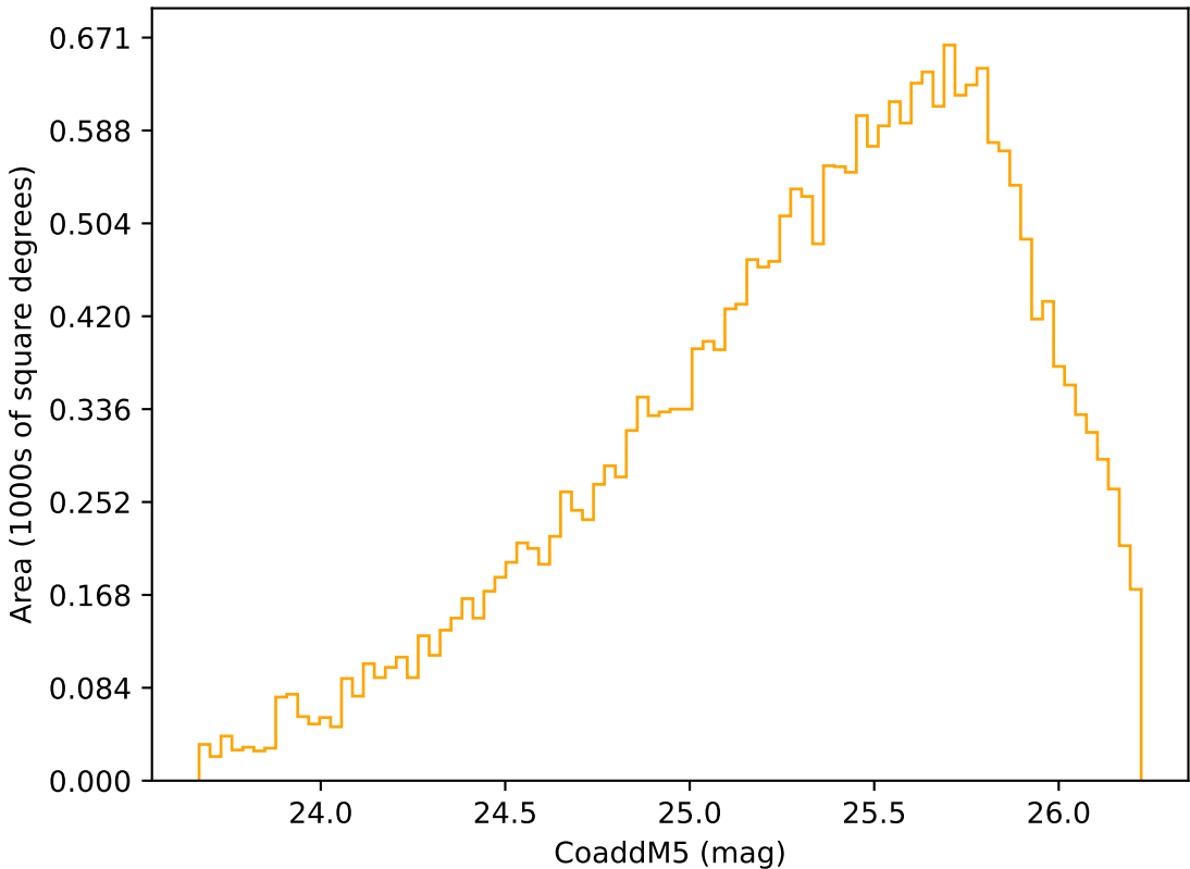
too_elab_2yr_r128_d3_griz_v3.4_10yrs Yr 3-4 r band: CoaddM5
