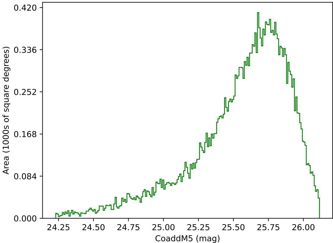
too_elab_2yr_r128_d3_griz_v3.4_10yrs Yr 1 g band: CoaddM5
