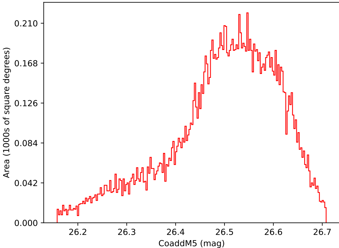
too_elab_2yr_r128_d3_griz_v3.4_10yrs WFD i band: CoaddM5
