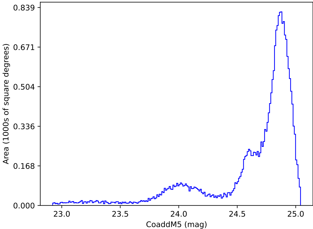
too_elab_2yr_r128_d3_griz_v3.4_10yrs All sky y band: CoaddM5
