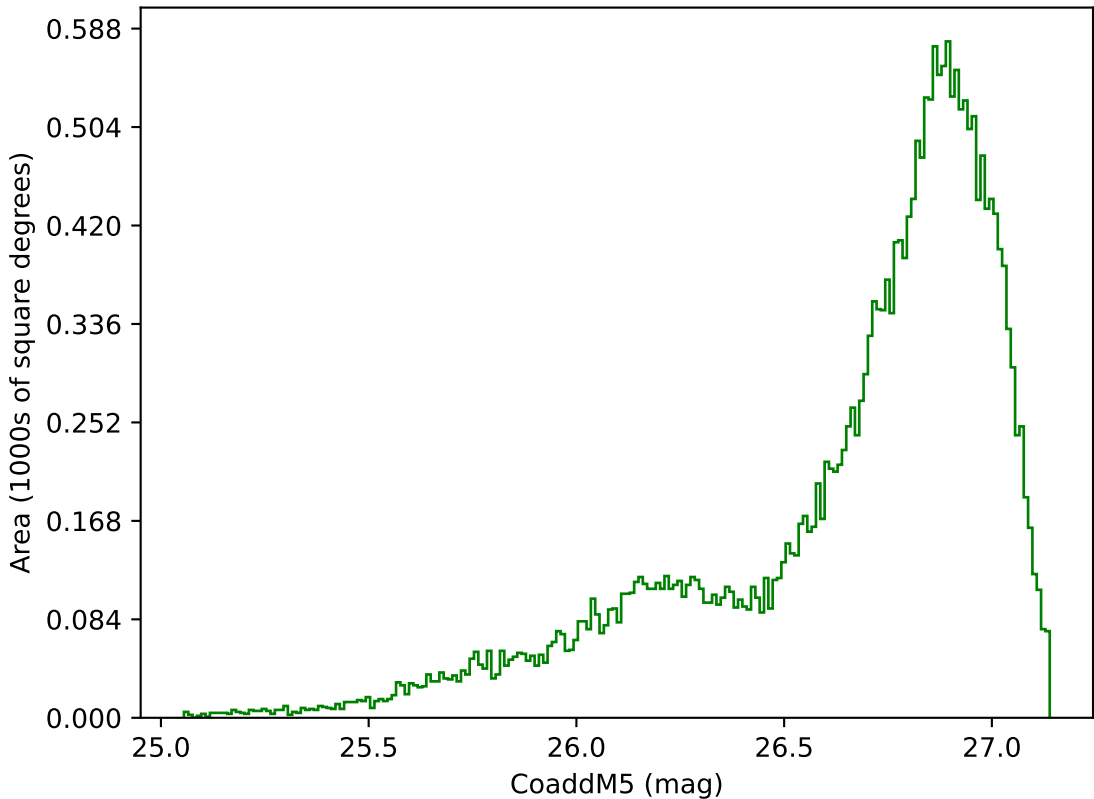
too_elab_2yr_r128_d3_griz_v3.4_10yrs All sky g band: CoaddM5
