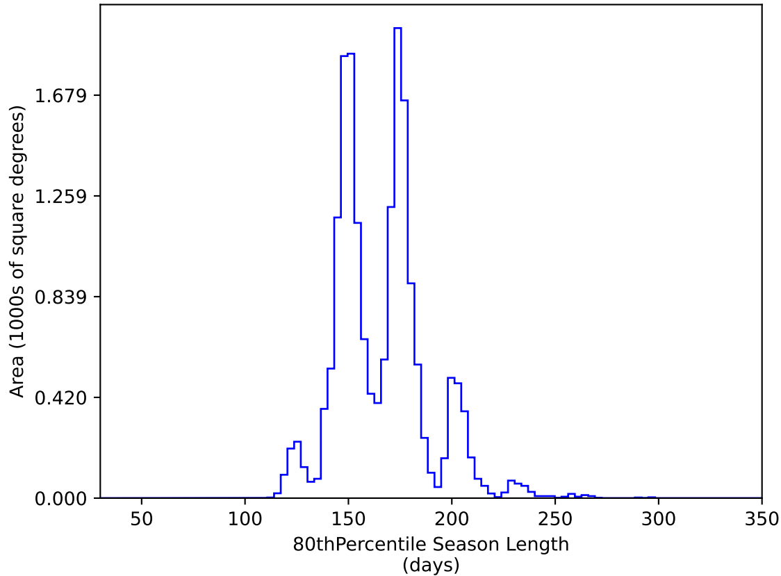
too_elab_2yr_r128_d3_griz_v3.4_10yrs WFD y band: 80thPercentile Season Length
