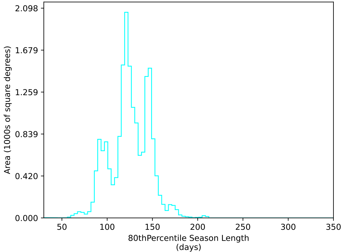
too_elab_2yr_r128_d3_griz_v3.4_10yrs WFD u band: 80thPercentile Season Length
