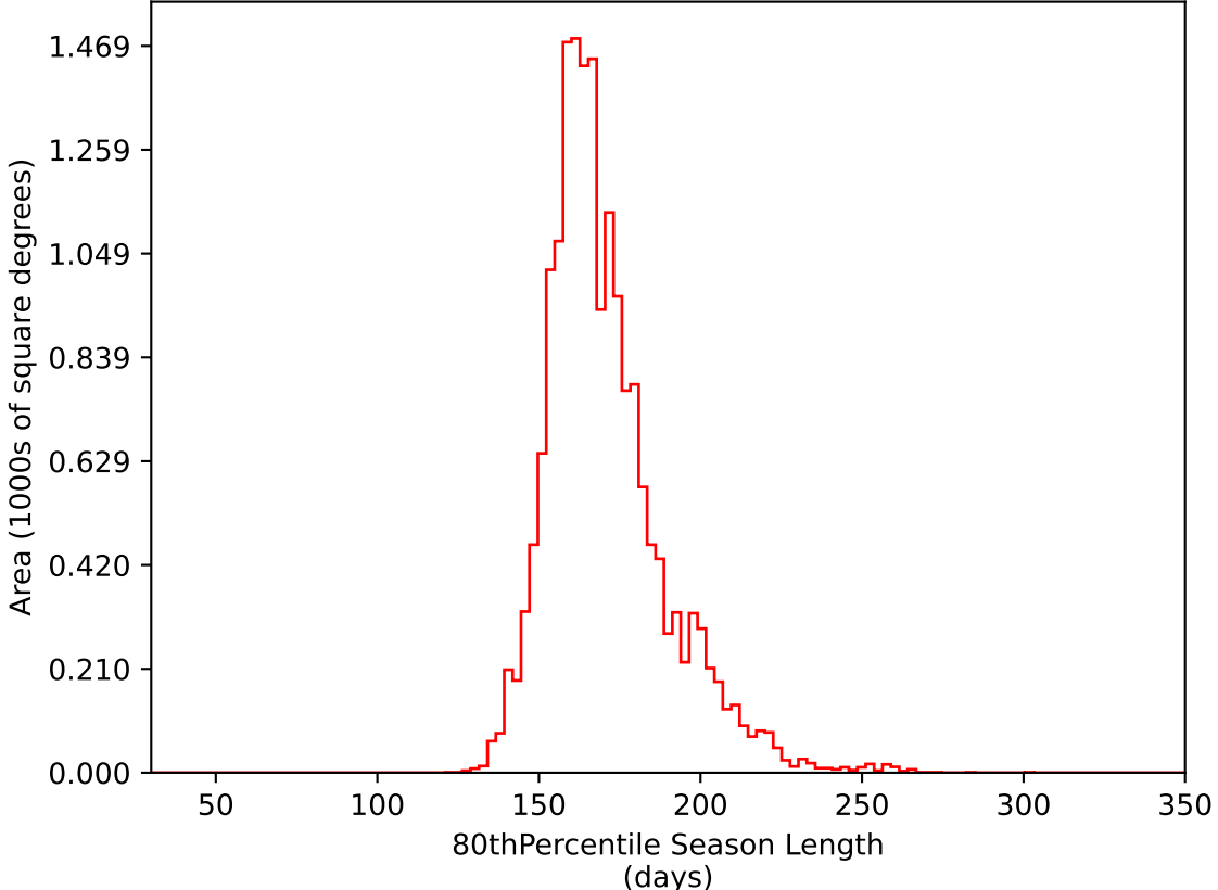
too_elab_2yr_r128_d3_griz_v3.4_10yrs WFD i band: 80thPercentile Season Length
