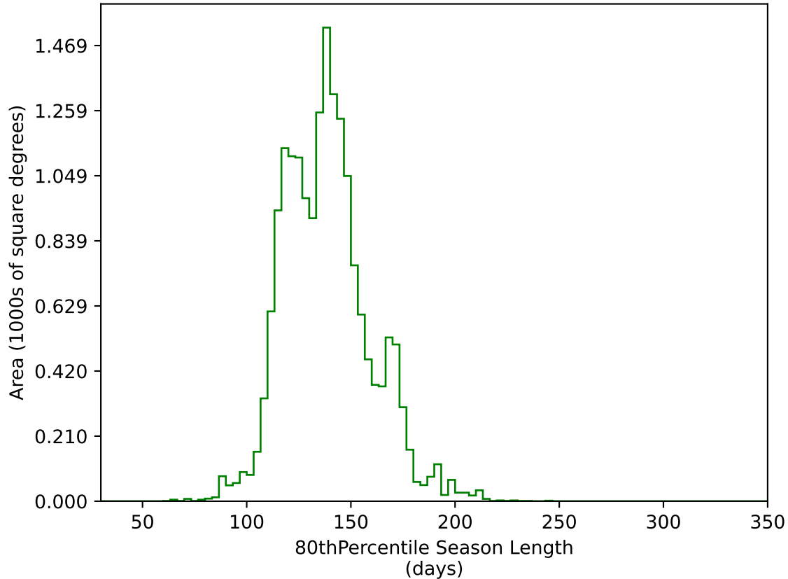
too_elab_2yr_r128_d3_griz_v3.4_10yrs WFD g band: 80thPercentile Season Length
