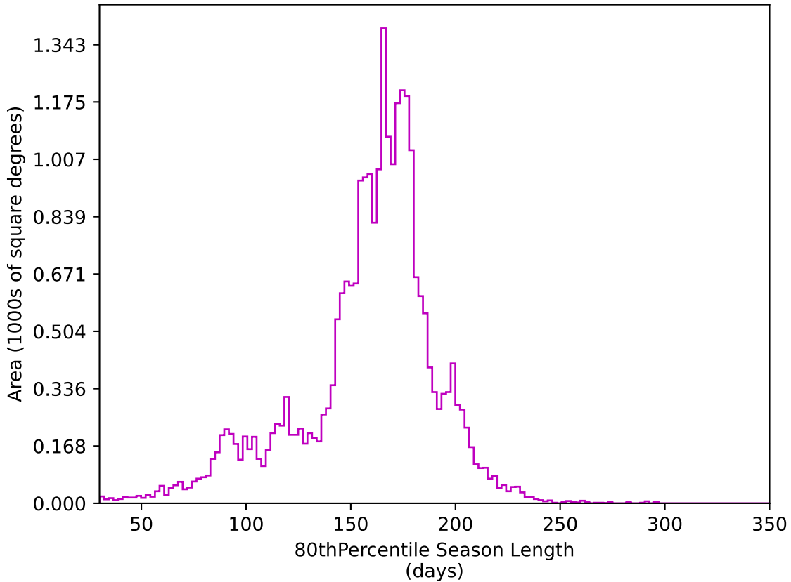
too_elab_2yr_r128_d3_griz_v3.4_10yrs All sky z band: 80thPercentile Season Length
