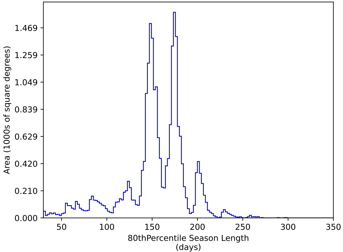
too_elab_2yr_r128_d3_griz_v3.4_10yrs All sky y band: 80thPercentile Season Length
