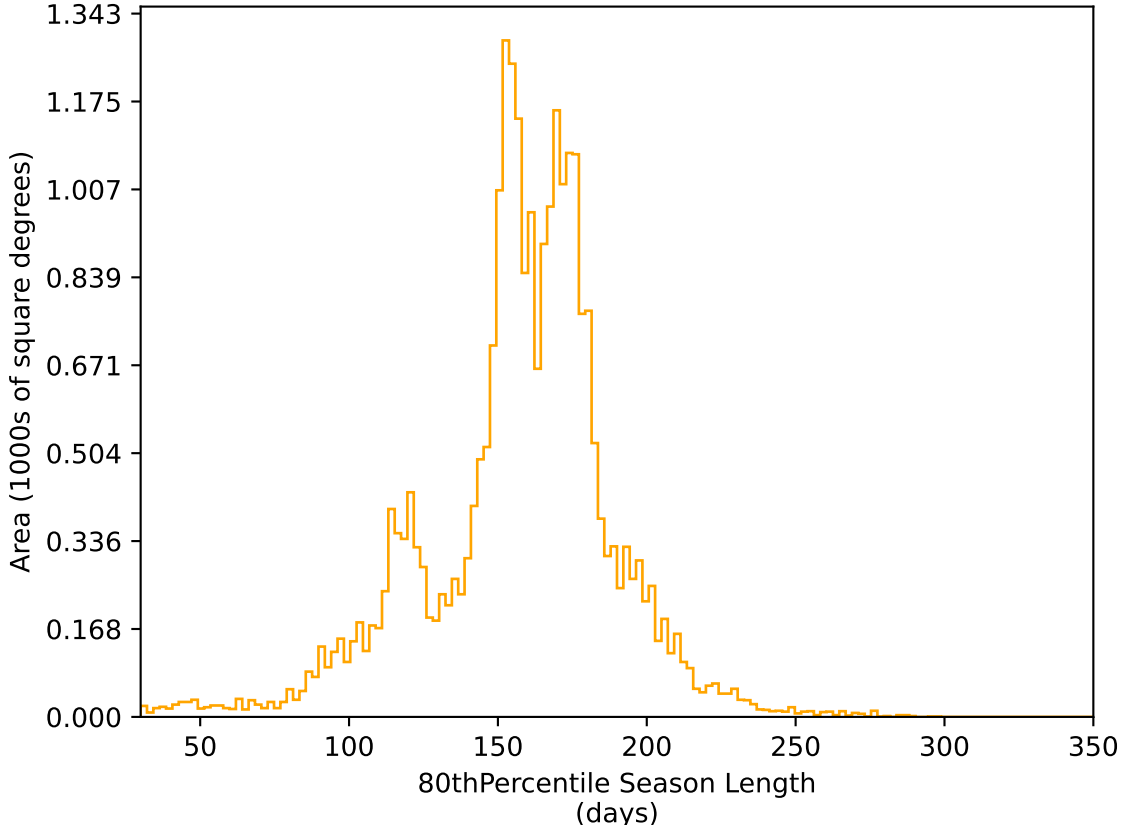
too_elab_2yr_r128_d3_griz_v3.4_10yrs All sky r band: 80thPercentile Season Length
