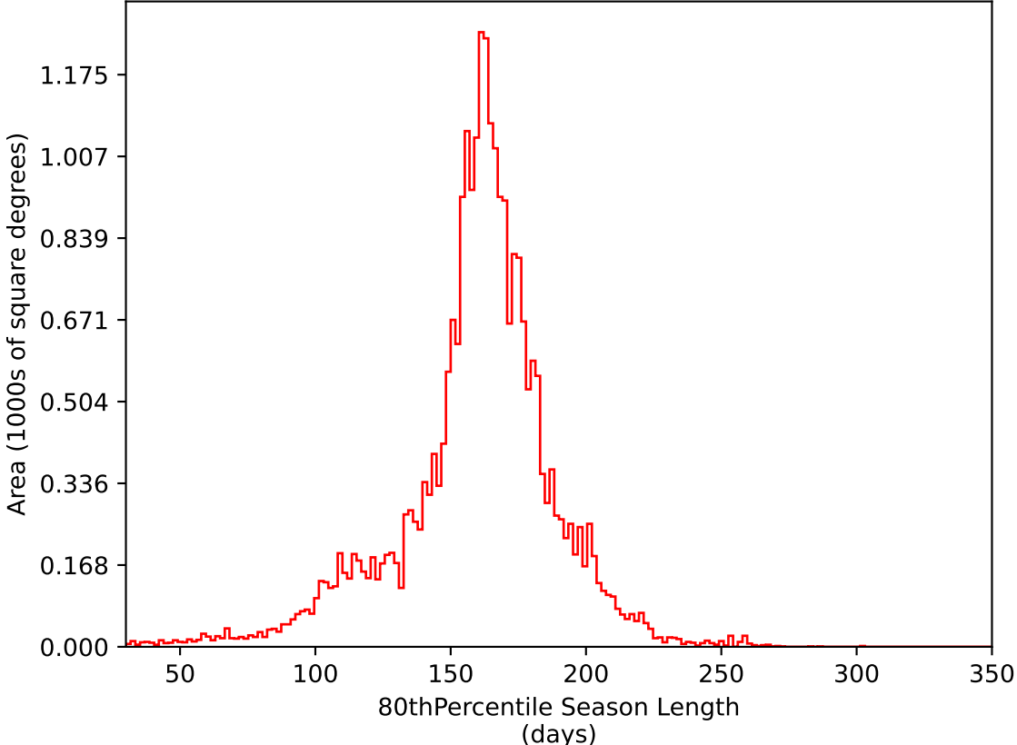
too_elab_2yr_r128_d3_griz_v3.4_10yrs All sky i band: 80thPercentile Season Length
