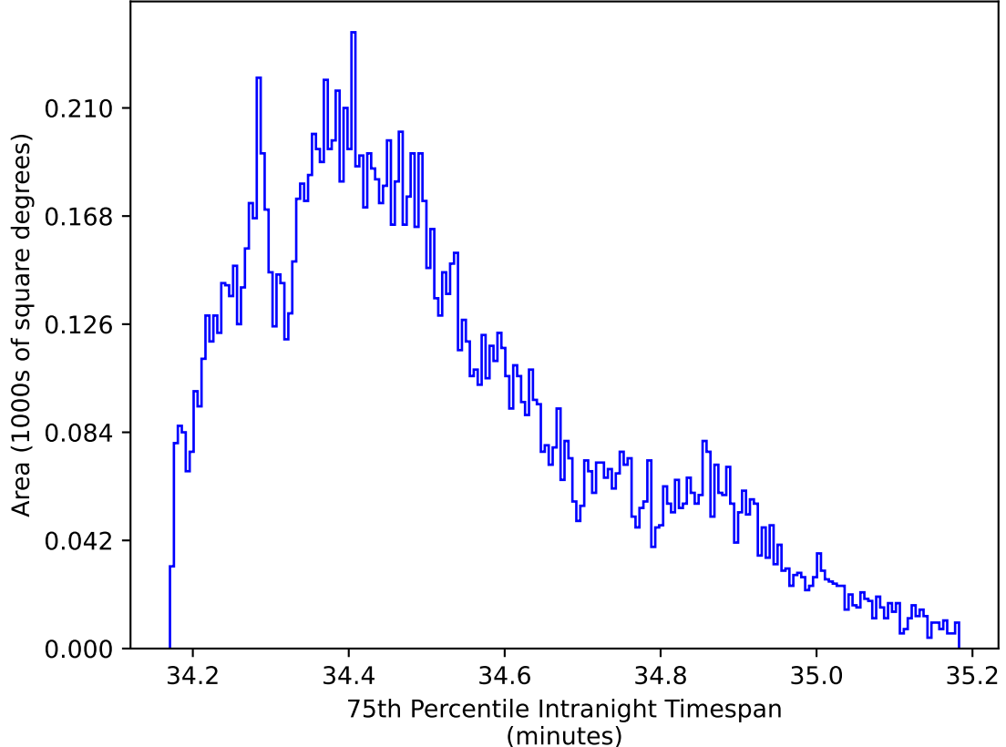
too_elab_2yr_r128_d3_griz_v3.4_10yrs WFD zy bands: 75th Percentile Intranight Timespan
