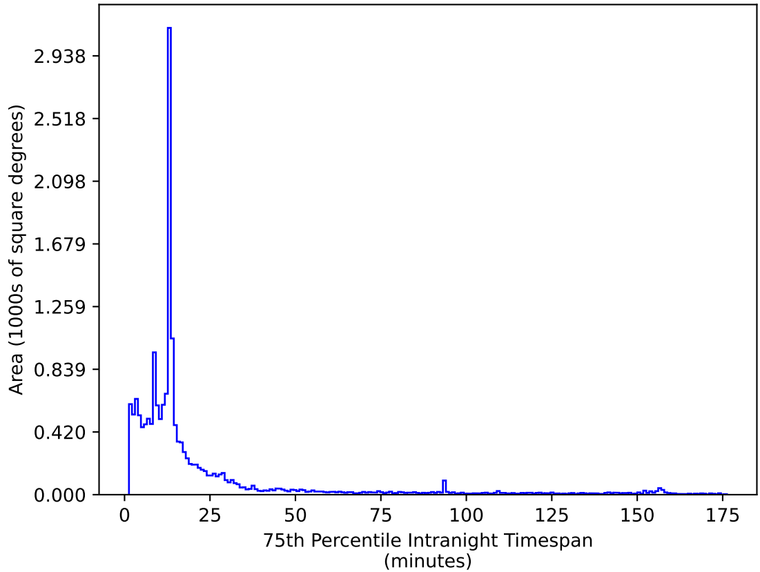
too_elab_2yr_r128_d3_griz_v3.4_10yrs WFD z band: 75th Percentile Intranight Timespan
