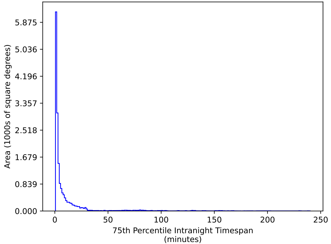
too_elab_2yr_r128_d3_griz_v3.4_10yrs WFD u band: 75th Percentile Intranight Timespan
