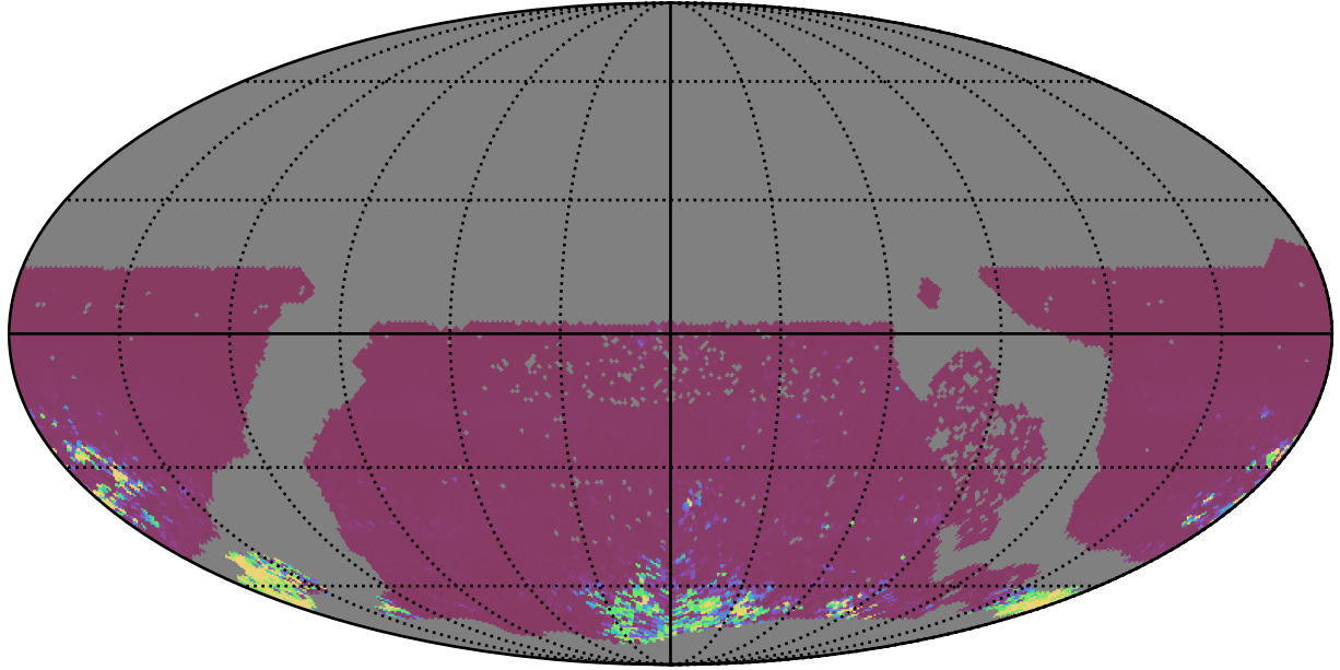
too_elab_2yr_r128_d3_griz_v3.4_10yrs WFD ri bands: 75th Percentile Intranight Timespan
