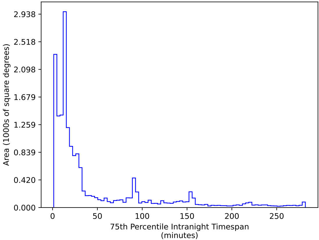
too_elab_2yr_r128_d3_griz_v3.4_10yrs WFD r band: 75th Percentile Intranight Timespan
