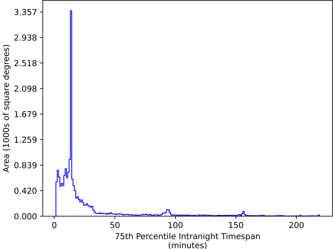
too_elab_2yr_r128_d3_griz_v3.4_10yrs WFD i band: 75th Percentile Intranight Timespan
