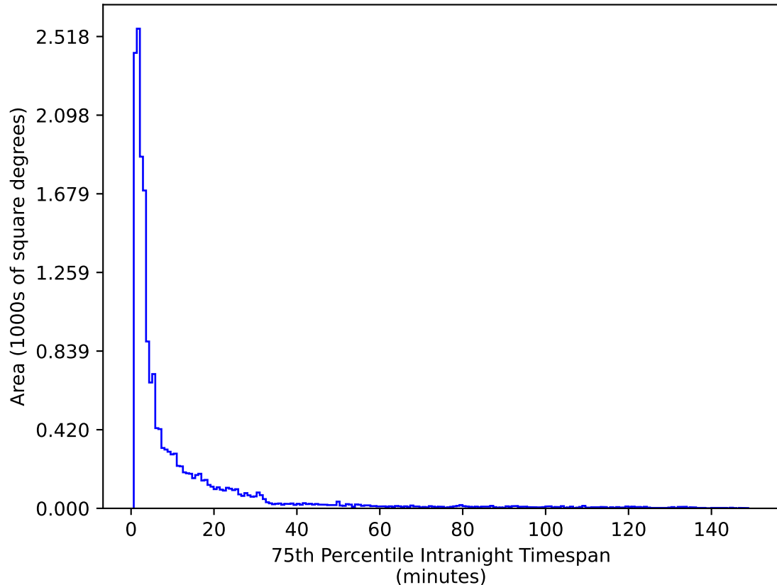
too_elab_2yr_r128_d3_griz_v3.4_10yrs WFD g band: 75th Percentile Intranight Timespan
