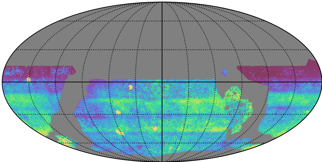
too_elab_2yr_r128_d3_griz_v3.4_10yrs WFD all bands: 75th Percentile Intranight Timespan
