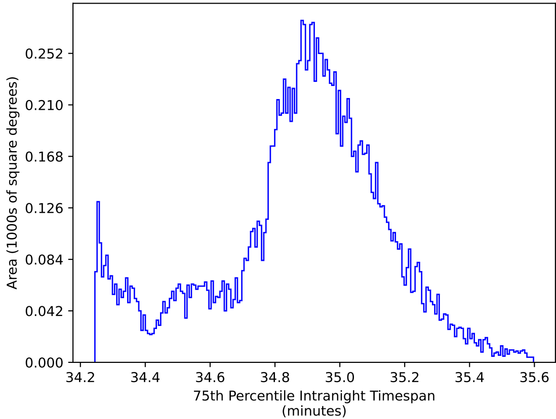
too_elab_2yr_r128_d3_griz_v3.4_10yrs WFD all bands: 75th Percentile Intranight Timespan
