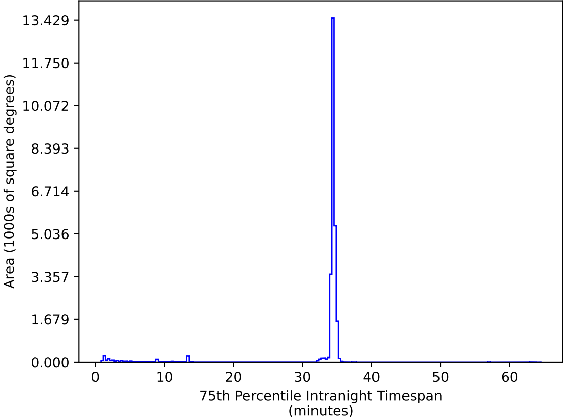
too_elab_2yr_r128_d3_griz_v3.4_10yrs All sky zy bands: 75th Percentile Intranight Timespan
