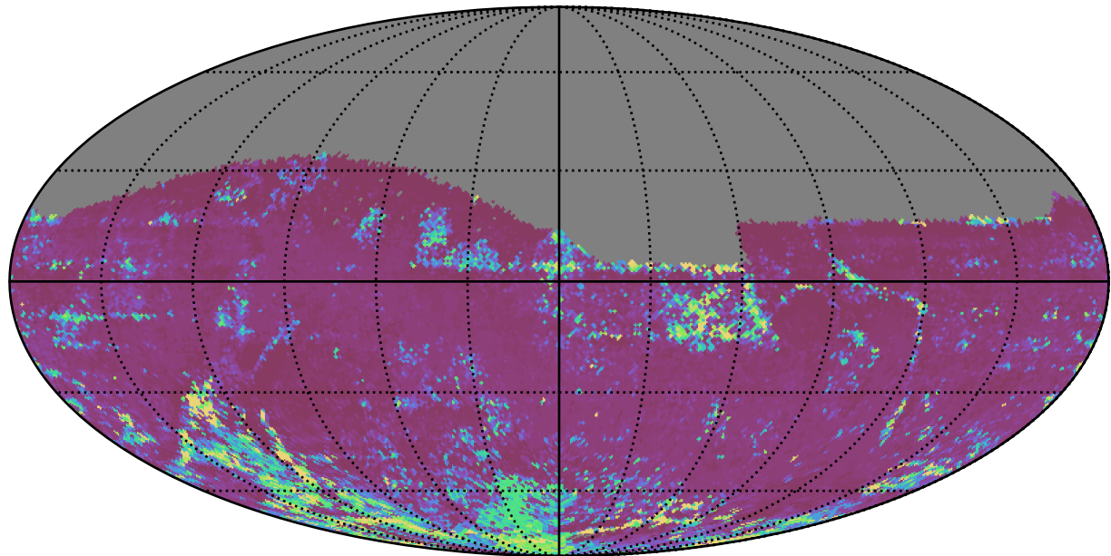
too_elab_2yr_r128_d3_griz_v3.4_10yrs All sky z band: 75th Percentile Intranight Timespan
