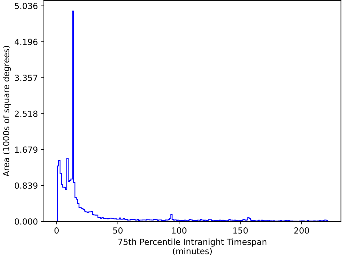
too_elab_2yr_r128_d3_griz_v3.4_10yrs All sky z band: 75th Percentile Intranight Timespan
