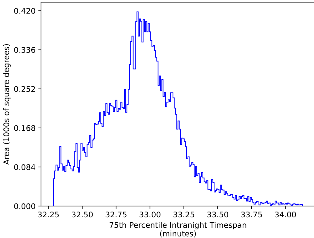
too_elab_2yr_r128_d3_griz_v3.4_10yrs All sky y band: 75th Percentile Intranight Timespan
