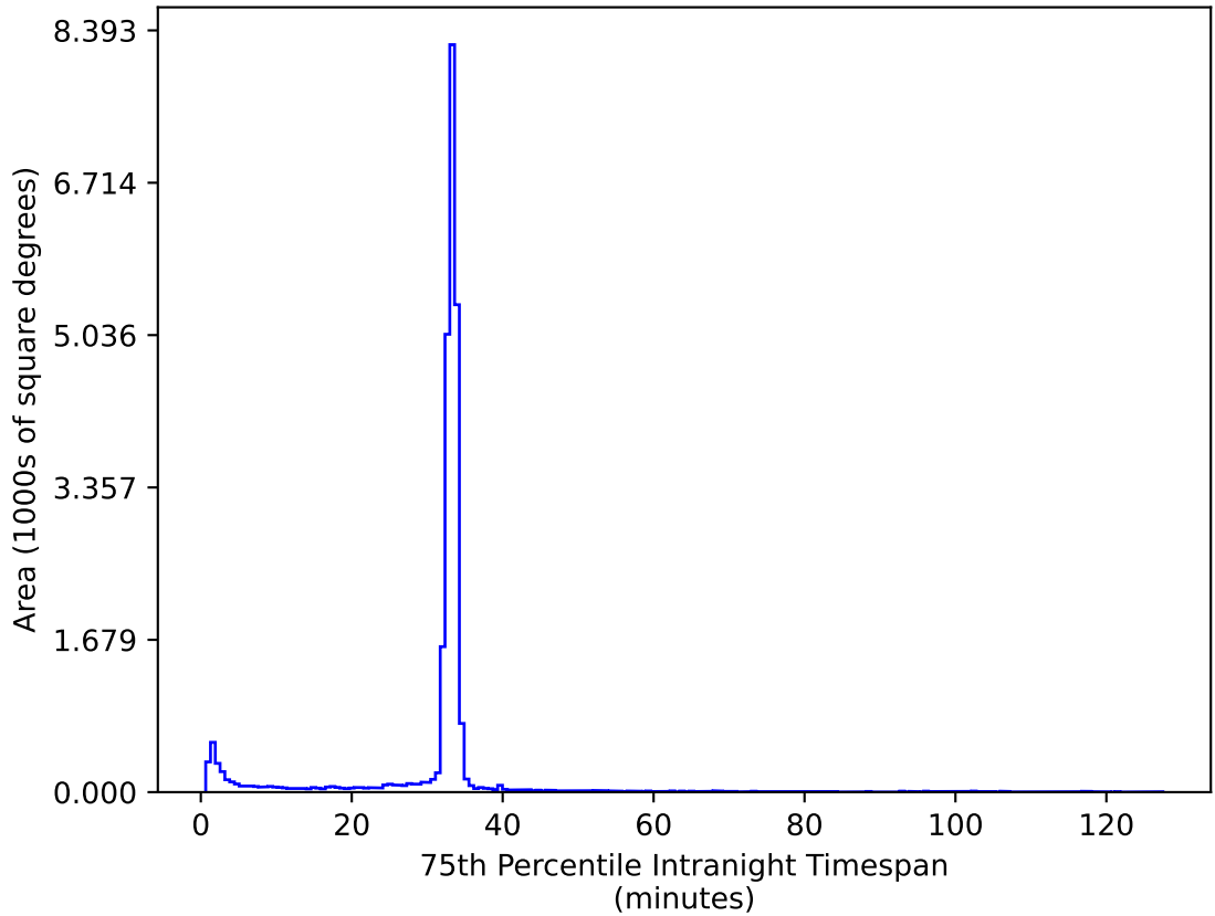
too_elab_2yr_r128_d3_griz_v3.4_10yrs All sky ug bands: 75th Percentile Intranight Timespan
