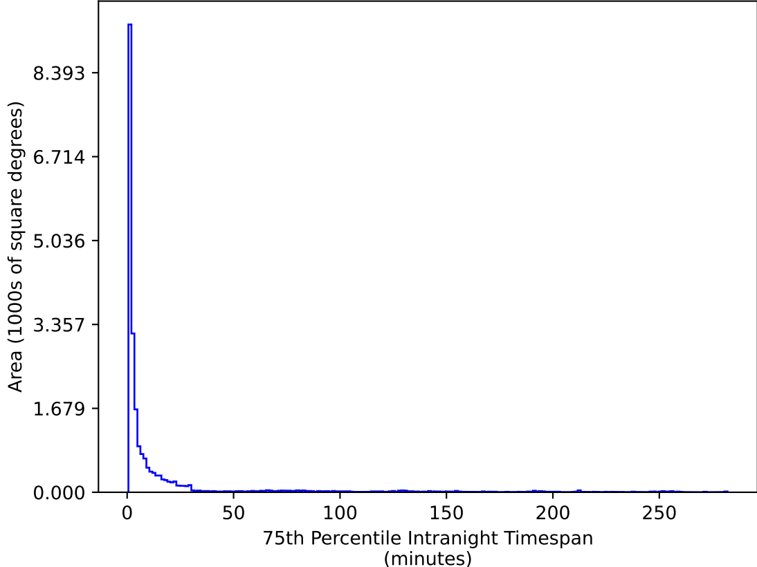
too_elab_2yr_r128_d3_griz_v3.4_10yrs All sky u band: 75th Percentile Intranight Timespan
