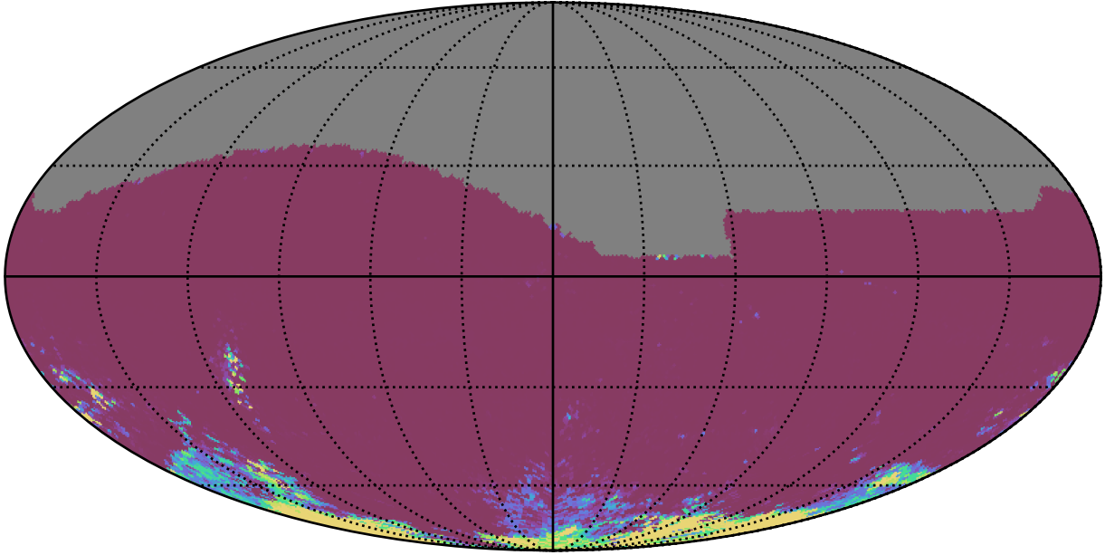
too_elab_2yr_r128_d3_griz_v3.4_10yrs All sky ri bands: 75th Percentile Intranight Timespan
