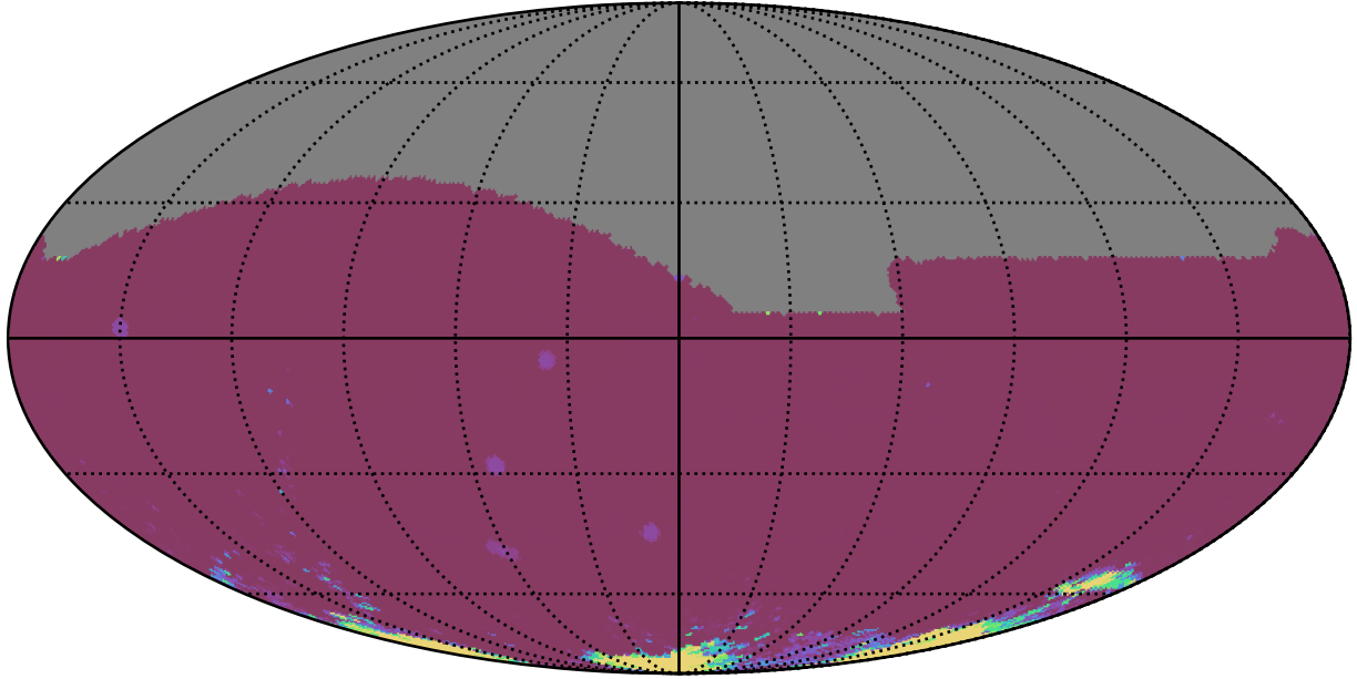
too_elab_2yr_r128_d3_griz_v3.4_10yrs All sky iz bands: 75th Percentile Intranight Timespan
