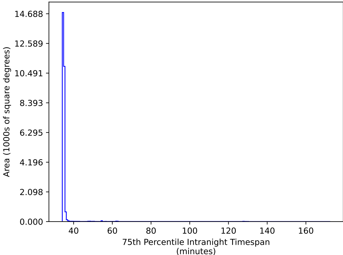
too_elab_2yr_r128_d3_griz_v3.4_10yrs All sky iz bands: 75th Percentile Intranight Timespan
