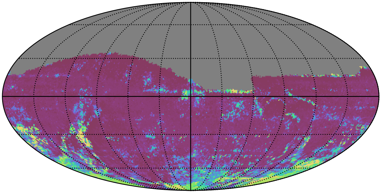
too_elab_2yr_r128_d3_griz_v3.4_10yrs All sky i band: 75th Percentile Intranight Timespan
