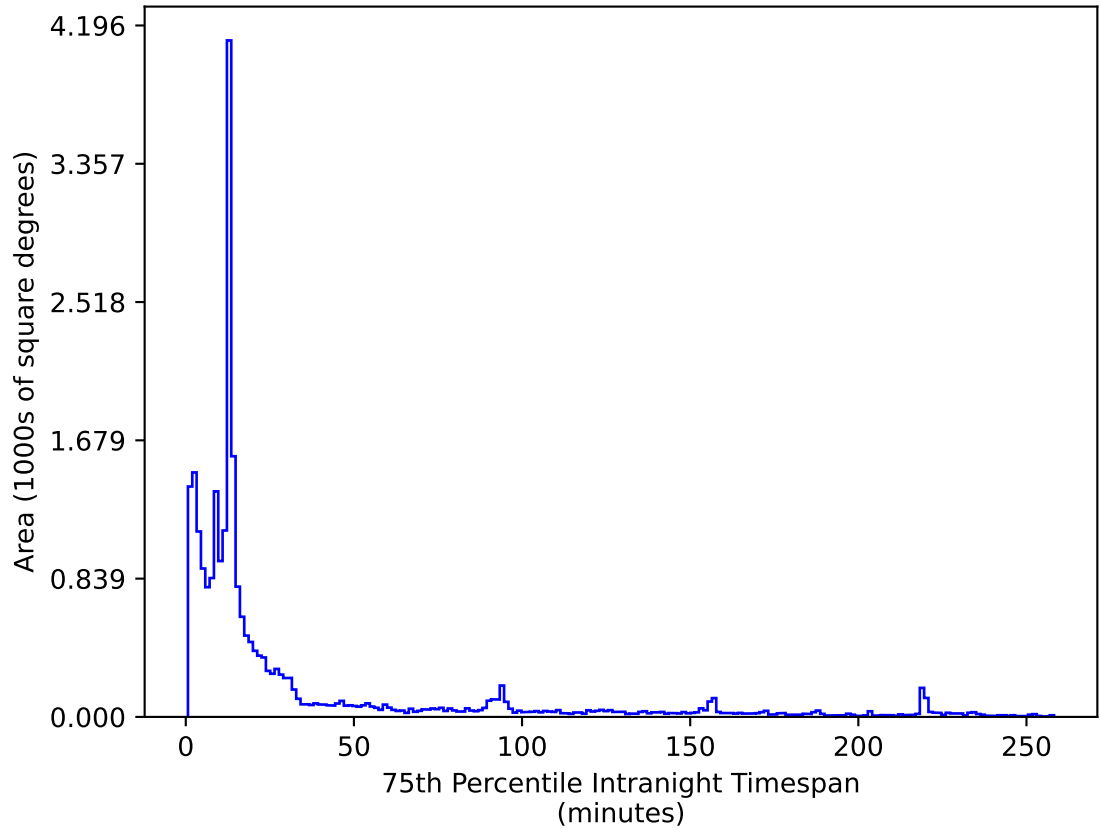
too_elab_2yr_r128_d3_griz_v3.4_10yrs All sky i band: 75th Percentile Intranight Timespan
