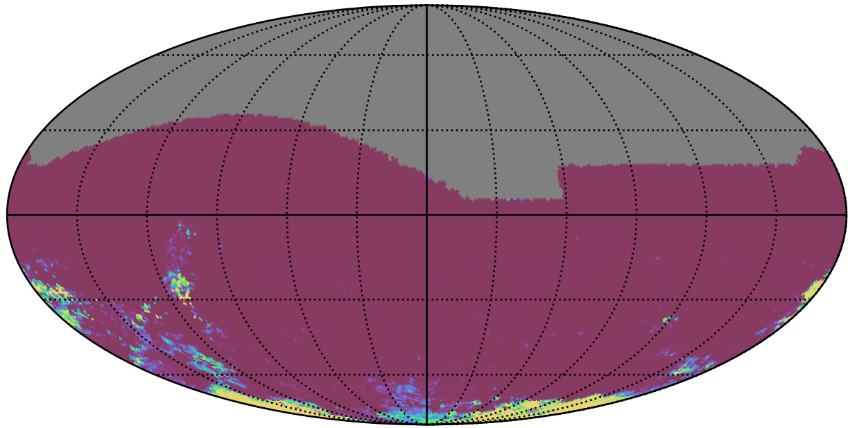
too_elab_2yr_r128_d3_griz_v3.4_10yrs All sky gr bands: 75th Percentile Intranight Timespan
